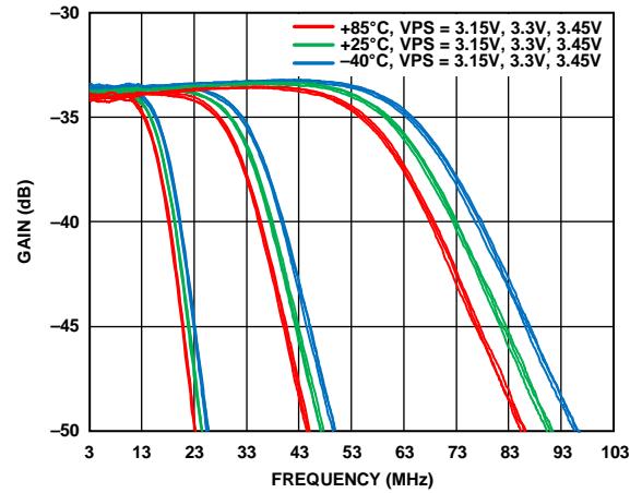
Figure 15. Frequency Response over Supply and Temperature; VGN1/VGN2/VGN3 = 0 V, Filter Corners = 15 MHz, 30 MHz, and 60 MHz
