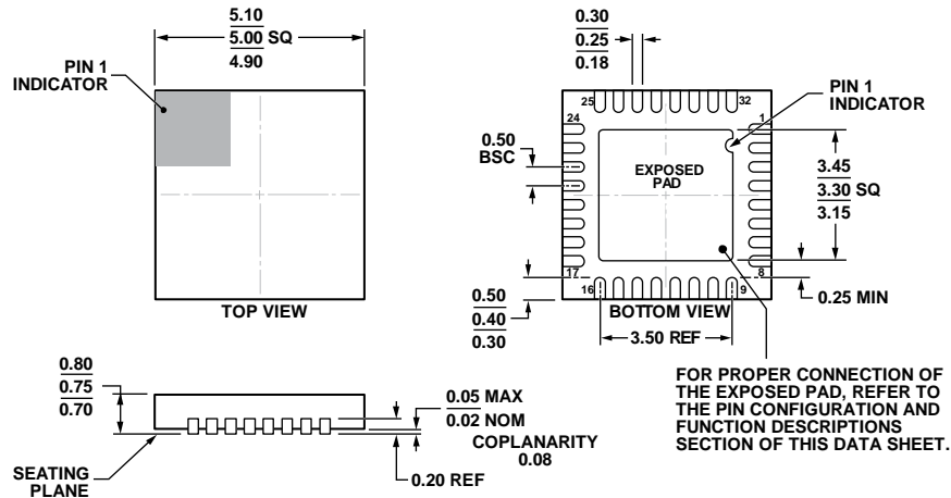
Figure 92. 32-Lead Lead Frame Chip Scale Package [LFCSP_WQ] 5 mm × 5 mm Body, Very Very Thin Quad (CP-32-13) Dimensions shown in millimeters
