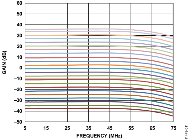
Figure 11. Gain vs. Frequency over VGN1/VGN2/VGN3
