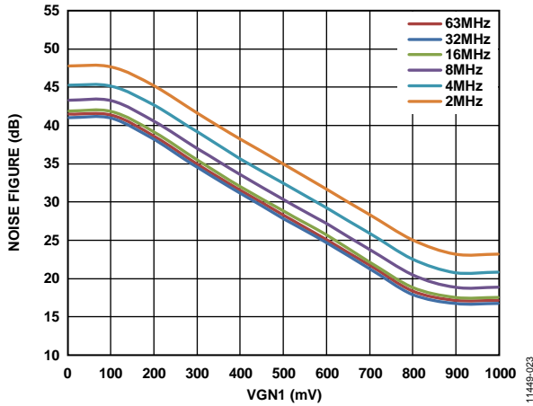
Figure 24. Noise Figure vs. VGN1 over Filter Corner; Digital Gain = 0000001, Noise Density Measured at Half of Filter Corner
