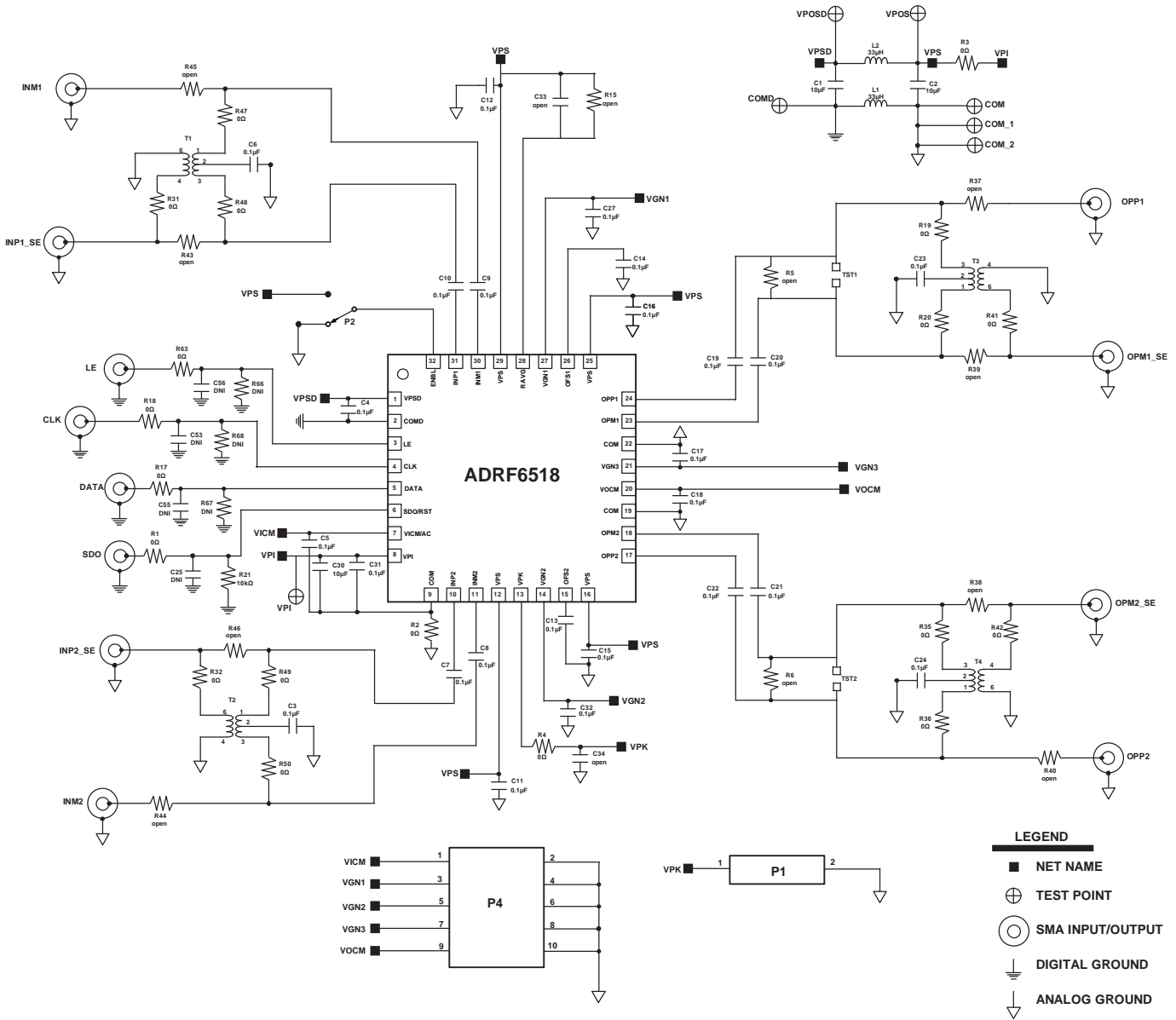
Figure 88. Evaluation Board Schematic
