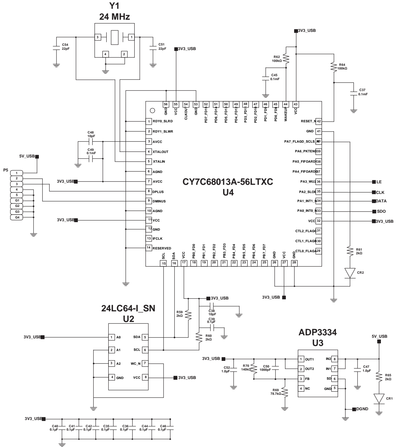
Figure 89. USB Evaluation Board Schematic
