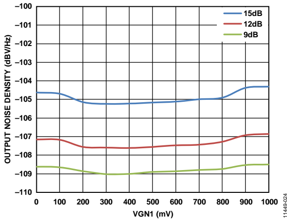
Figure 25. Output Noise Density vs. VGN1 over VGA1 Digital Gain; Noise Density Measured at Half of Filter Corner
