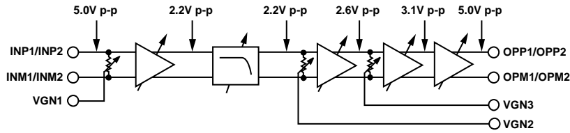
Figure 86. Maximum Signal Levels; Single Channel Shown
