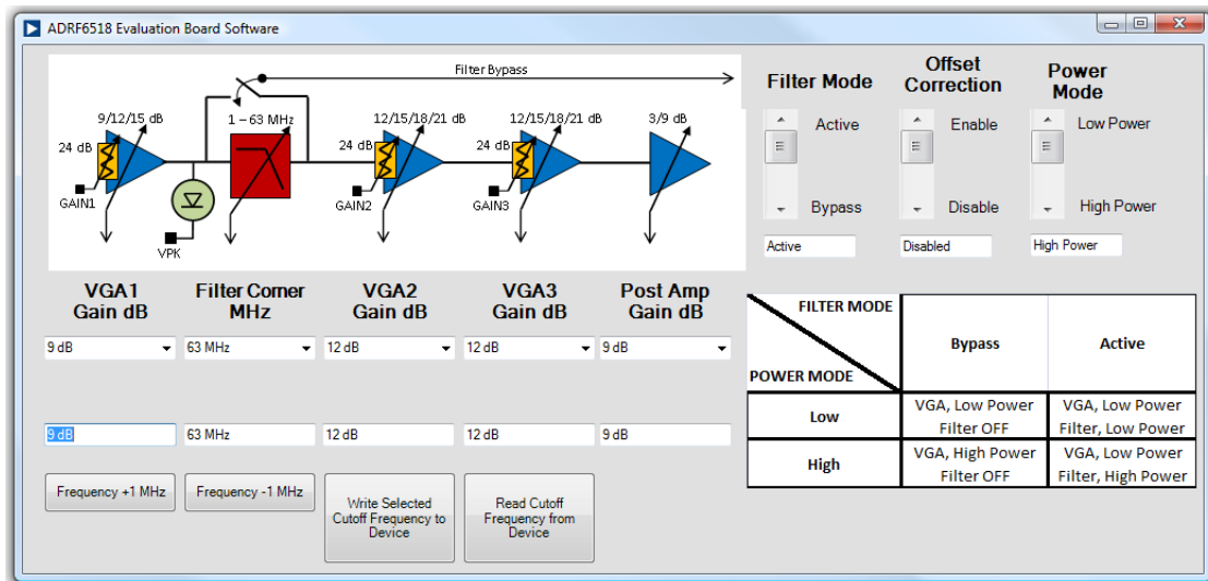
Figure 87. Analog Devices ADRF6518 Evaluation Software
